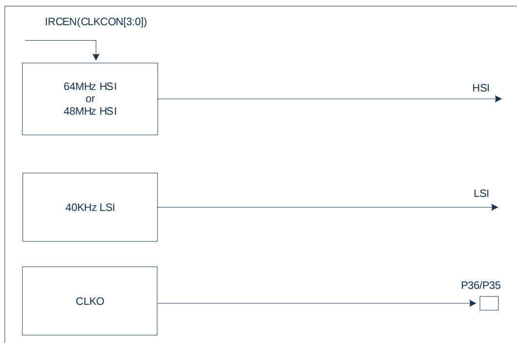
Figure 3-1: Block diagram of the clock structure
