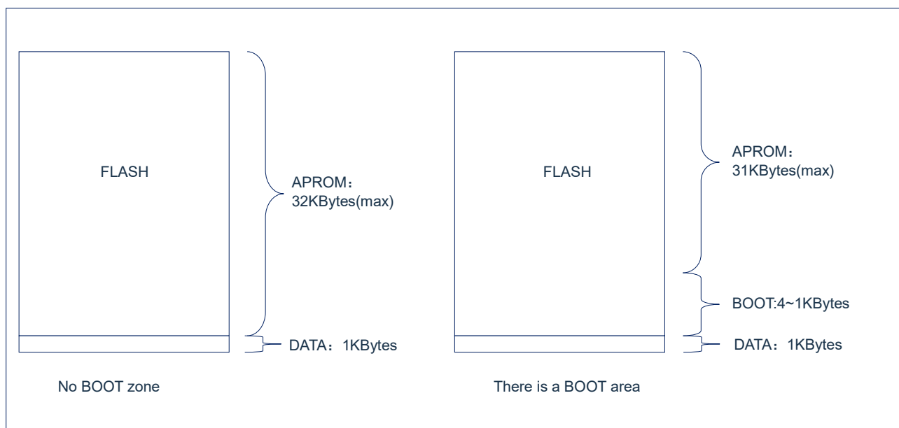
Figure 24-1: Storage structure diagram
